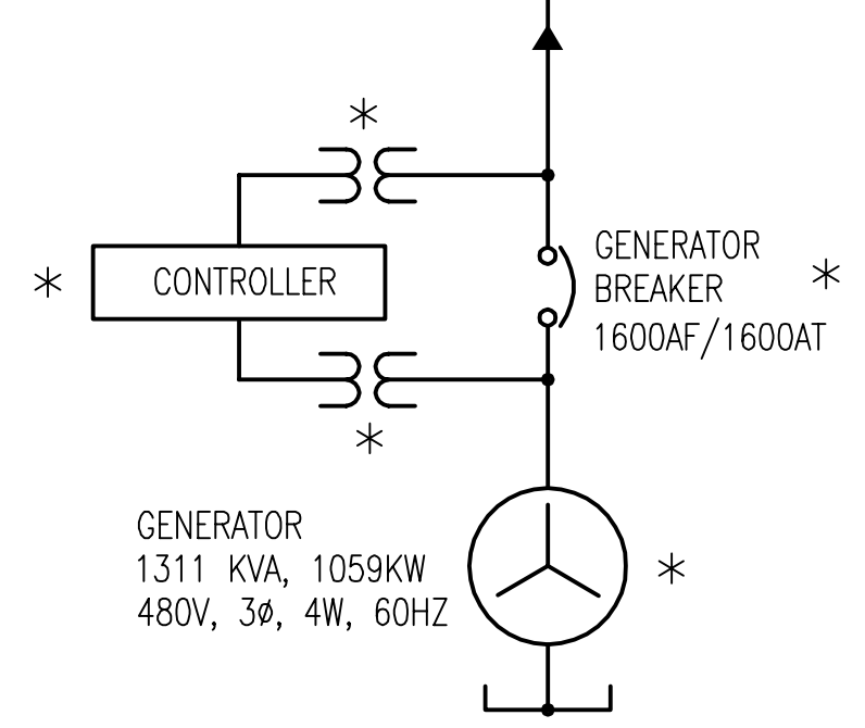
SINGLE LINE DIAGRAM NOT TO SCALE
